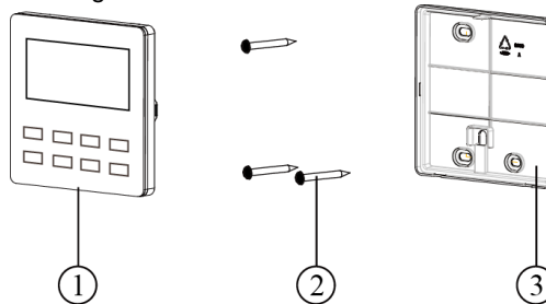
Fig. 22 Parts of wired controller
